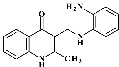
Figure. The structural formula of 3-[(2-aminoanilino)methyl]-2-methyl-1H-quinoline-4-one
