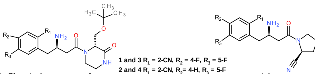
Fig. 1. Chemical structures of hypoglycemic agents as dpp-4 inhibitors
